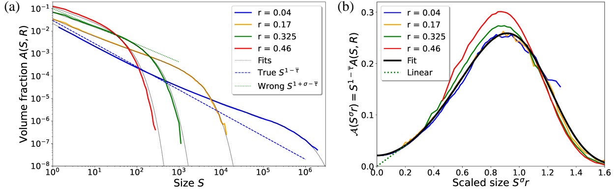
FIG. 1. Power laws and avalanche sizes in a random-field Ising model under an increasing field. [6] (a) Avalanche probability distribution A(S, R) that a site is in an avalanche of size S , for disorder R . Data are plotted at different values of r = (R - R_c)/R , where R_c is the critical disorder. The true power-law exponent is 1 - \bar{\tau} ; the apparent (wrong) power-law exponent is 1 + \sigma - \bar{\tau} . Note that one needs over four decades of scaling to discover the correct power law. (b) Scaling collapse of the same data, together with a fit to the scaling function \mathcal{A}(S^\sigma r) . Corrections to scaling are responsible for the deviations far from r = 0 . Note that one needs simulations of a billion spins to discover that the asymptote of \mathcal{A} was non-zero: smaller simulations gave the wrong power law given by the dotted lines. Data reproduced from [6].
