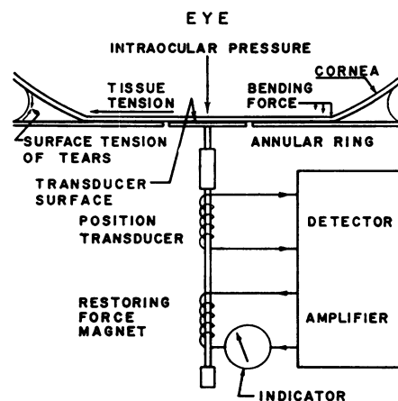
Fig. 1. If the cornea of the eye is flattened against a probe to beyond the pressure sensitive region then the only force that will be recorded will be intraocular pressure, since such factors as corneal rigidity exercise their force beyond the periphery of the sensitive region. Any tendency towards motion in the displacement transducer is detected and amplified to produce a restoring force that holds the pressure sensing piston coplaner with the surrounding region. The restoring-force current is recorded as a measure of intraocular pressure.
