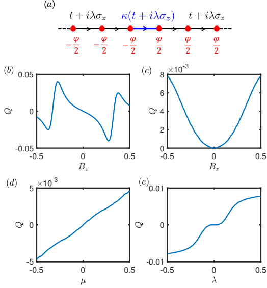
FIG. 1. (a) Scheme of the superconducting chain along \hat{x} -direction. The hopping amplitude t and the SOC strength \lambda are reduced by a factor \kappa on the interface (blue) bond. The superconducting phases on the two leads are \pm\varphi/2 . In numerical calculations, the length of each lead is set to 64 lattice sites. From (b) to (e), the nonreciprocal factor Q defined in Eq. (10) is plotted with varying B_z , B_x , \mu and \lambda , respectively, while keeping the others fixed at B_z = B_x = \lambda = 0.5 , \mu = 1 , \Delta = 0.2 and \kappa = 0.4 .
