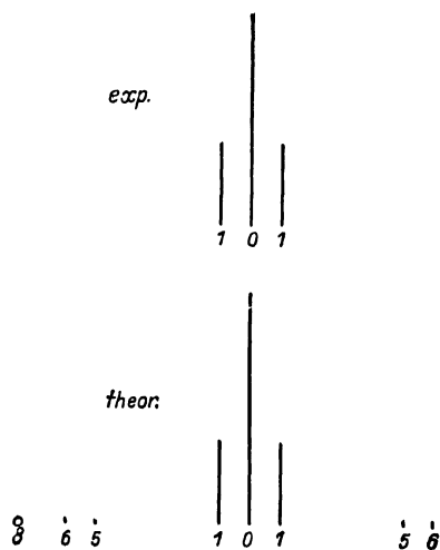
FIG. 2.— H_\alpha \perp -components
