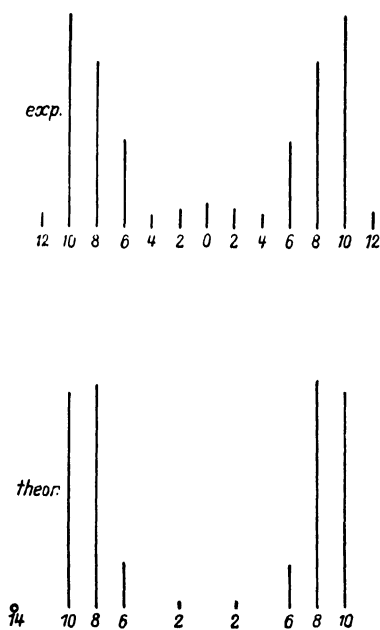
FIG. 3.— H_\beta ||-components.
