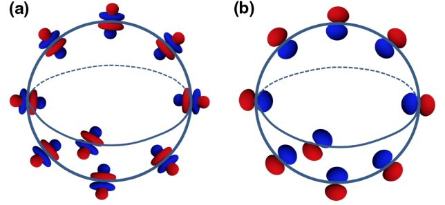
FIG. 1. Pictorial representations of the pairing matrices over the Fermi surfaces of (a) the isotropic f -wave septet pairing and (b) the isotropic p -wave triplet pairing with spin- \frac{3}{2} fermions. Intuitively, the f -wave matrix kernels U(\hat{k})S^{30}U^\dagger(\hat{k}) and the p -wave ones U(\hat{k})S^{10}U^\dagger(\hat{k}) for each wave vector \hat{k} are depicted in their orbital counterpart harmonic functions in (a) and (b), respectively.
