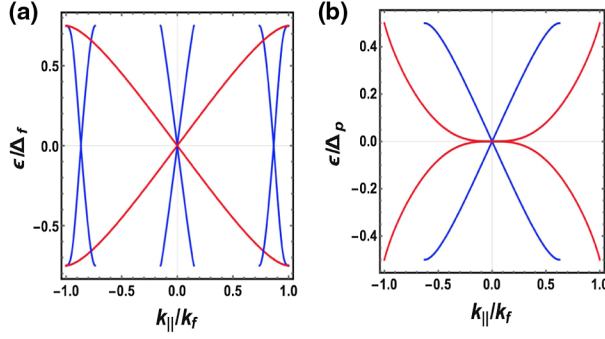
FIG. 2. The gapless surface spectra for the isotropic f -wave septet pairing in (a) and for the isotropic p -wave triplet pairing in (b) with spin- \frac{3}{2} fermions.
